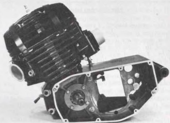
The entire transmission can be removed without splitting the cases. The lever hanging out in the opening is the engagement lever for first gear.
