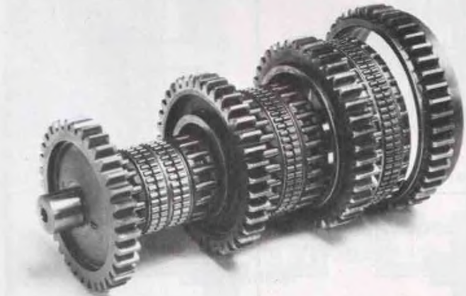
The rear gear cluster disassembled looks like this. Each shaft has two roller bearings separated by a freewheeling device. The narrowest shaft has two freewheeling devices because they couldn't get enough dogbones into one device to absorb the engine's load.
